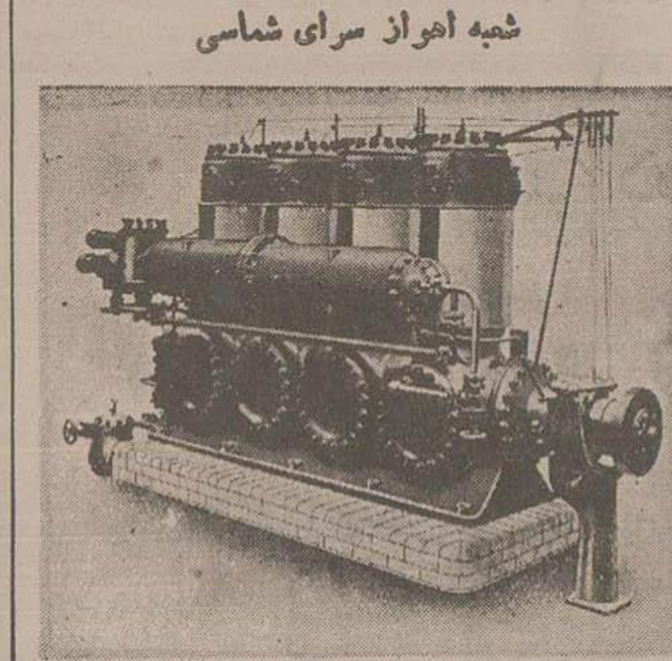
Four-Cylinder mark 4 Z 12 Ammonia compressor
