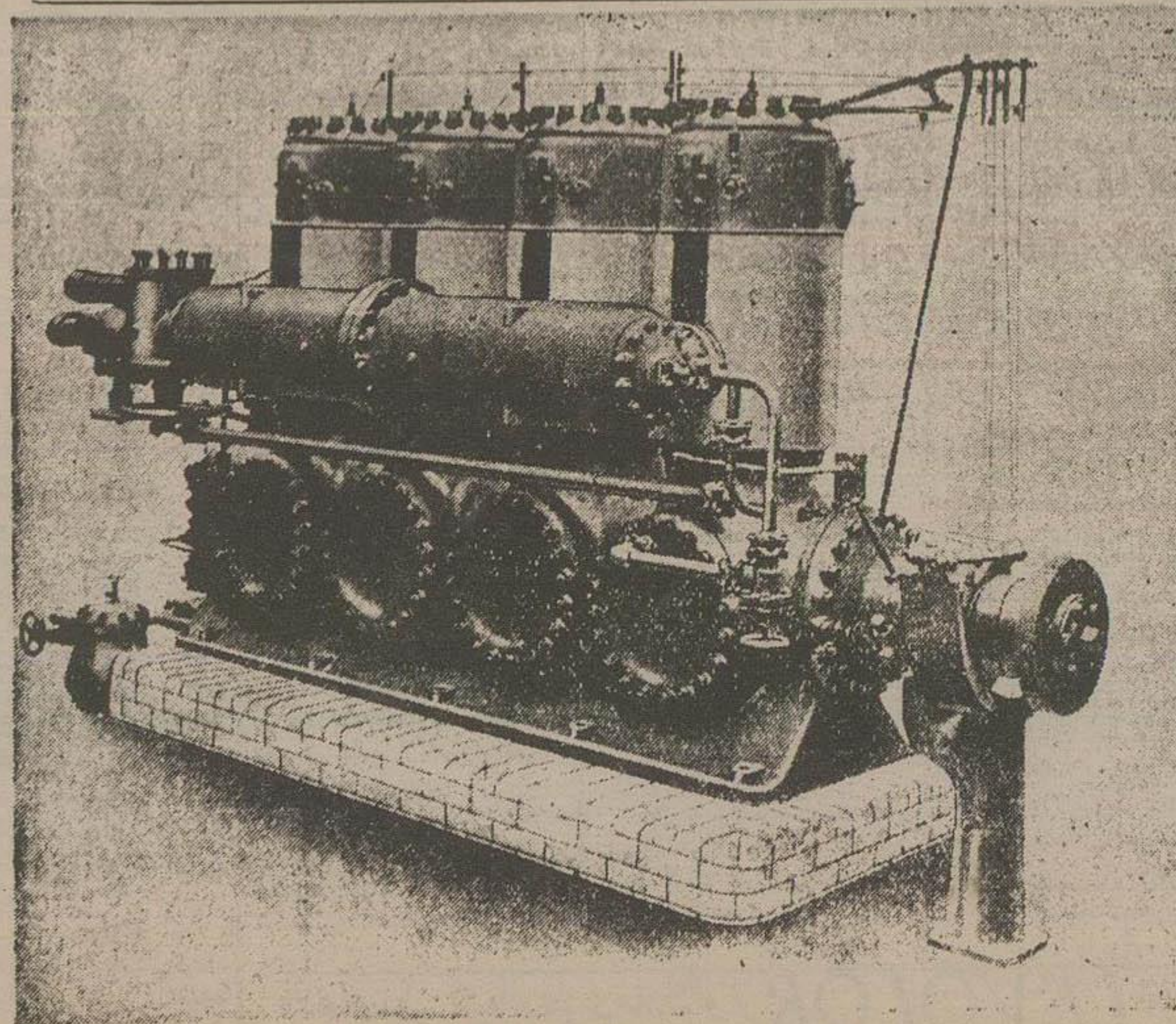
Four-Cylinder Mark 4z12 Ammonia Compressor
