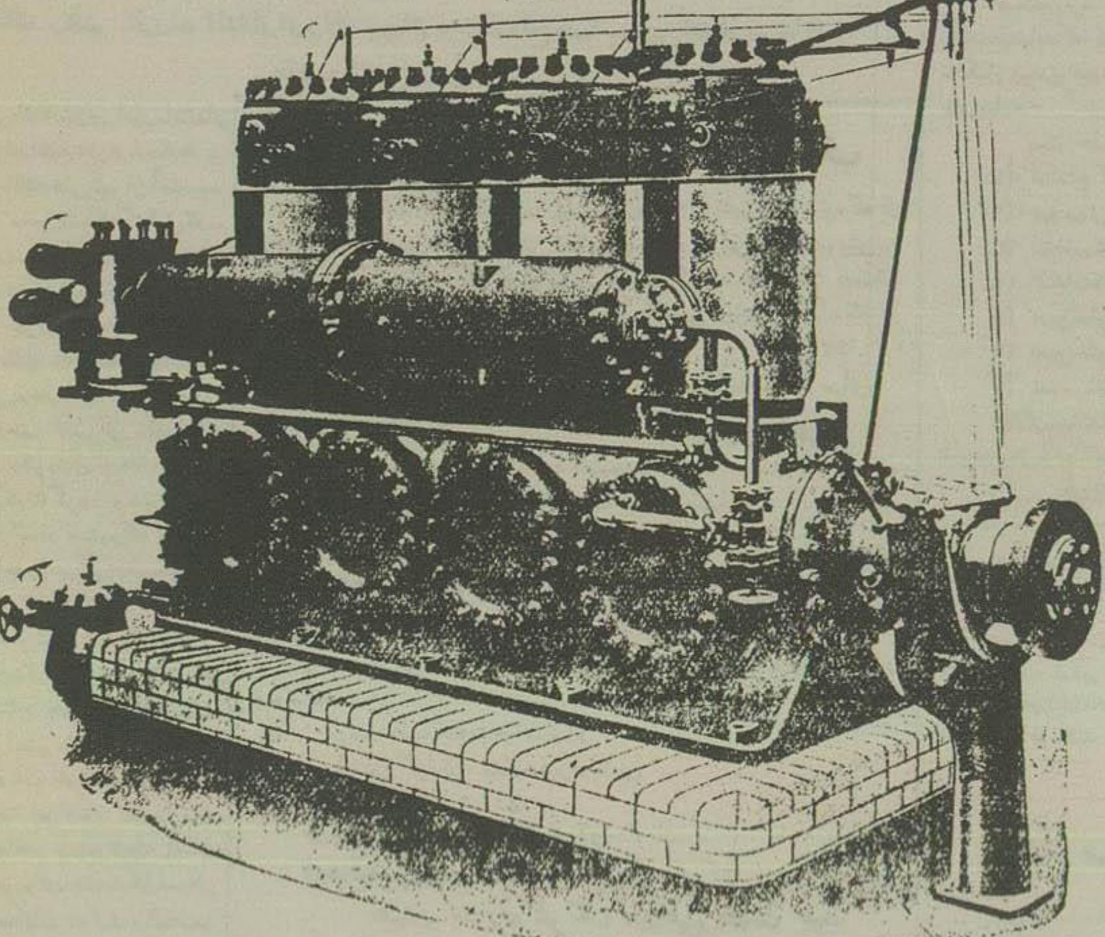
Four Cylinder mark 4 Z 12 Ammonia compressor. Rated capacity 220 tons refrigeration at 300 R.P.M.
