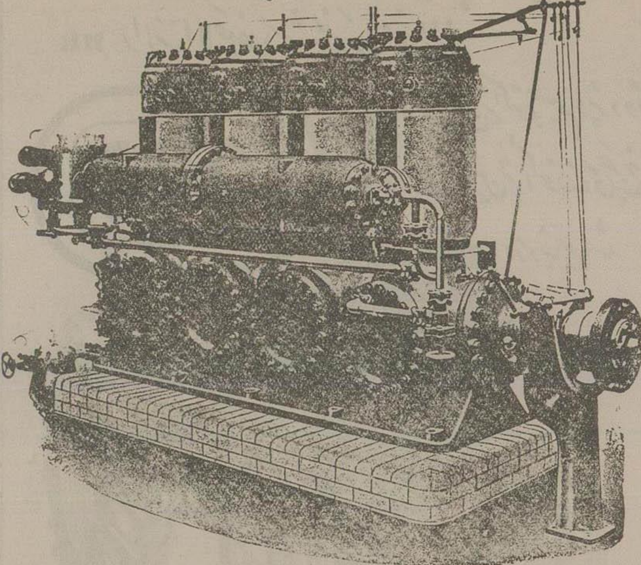
Four-Cylinder Mark 4Z12 Ammonia Compressor. Rated capacity 220 tons refrigeration at 300 r.p.m.
